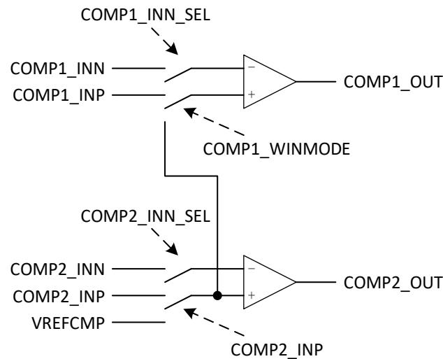
图 13-2 window comparator
